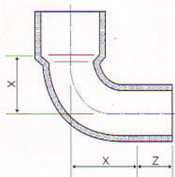
90° ELBOW B
